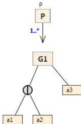
Figure 6.8: Group with Fixed Size
