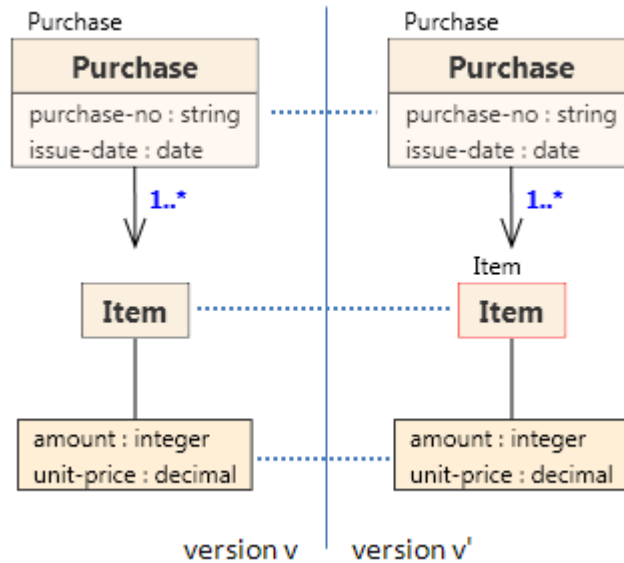
(a) Adding element label
