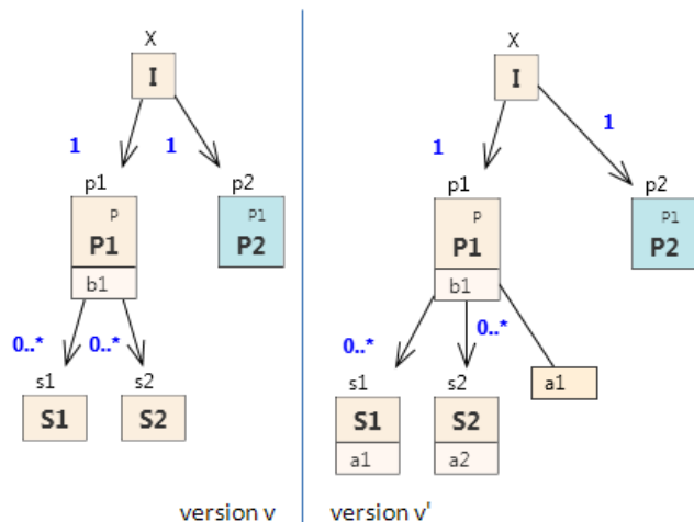
Figure 6.14: Match Attribute of Top Level Templates
