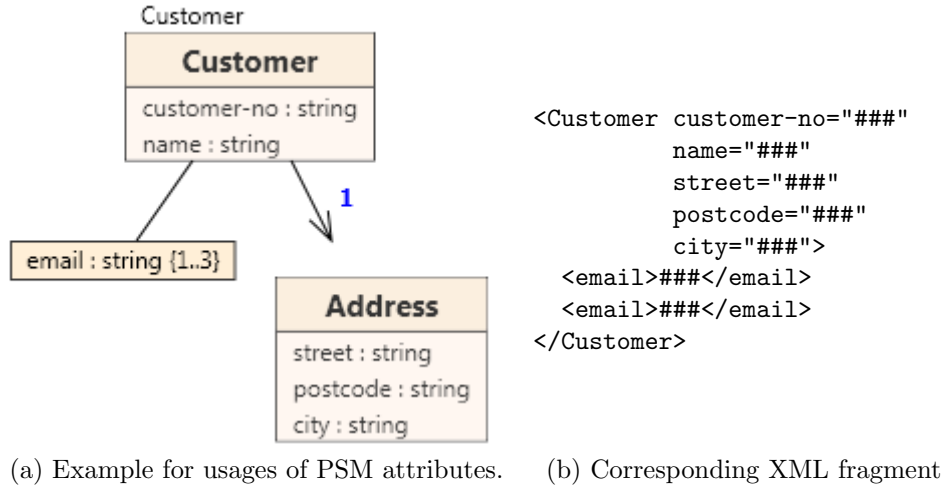
Figure 3.9: PSM Attributes, an Attribute Container and a Corresponding XML Fragment
